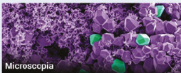
Microscopia
