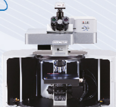
Raman
